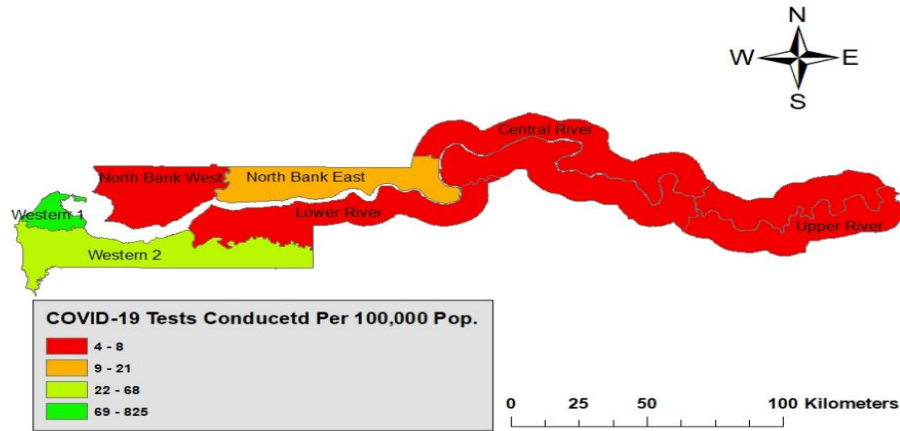
Fig 2: Geographic Distribution of Recent Tests Conducted Per 100,000 Pop. by Region, March 16-14 April 2021
