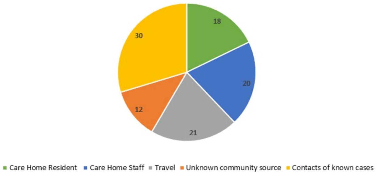
Case grouping (%)
