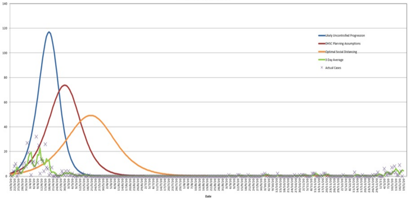
Daily Confirmed Cases
