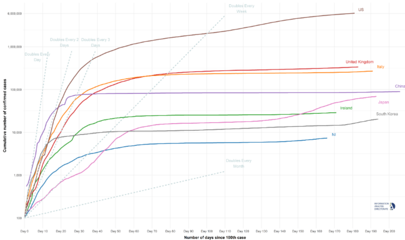
Figure 1: Cumulative number of individuals with a laboratory confirmed test for COVID-19 after the 100 th case.
