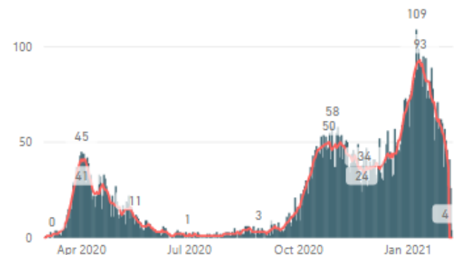
Confirmed COVID-19 daily admissions (South Eastern Trust)
