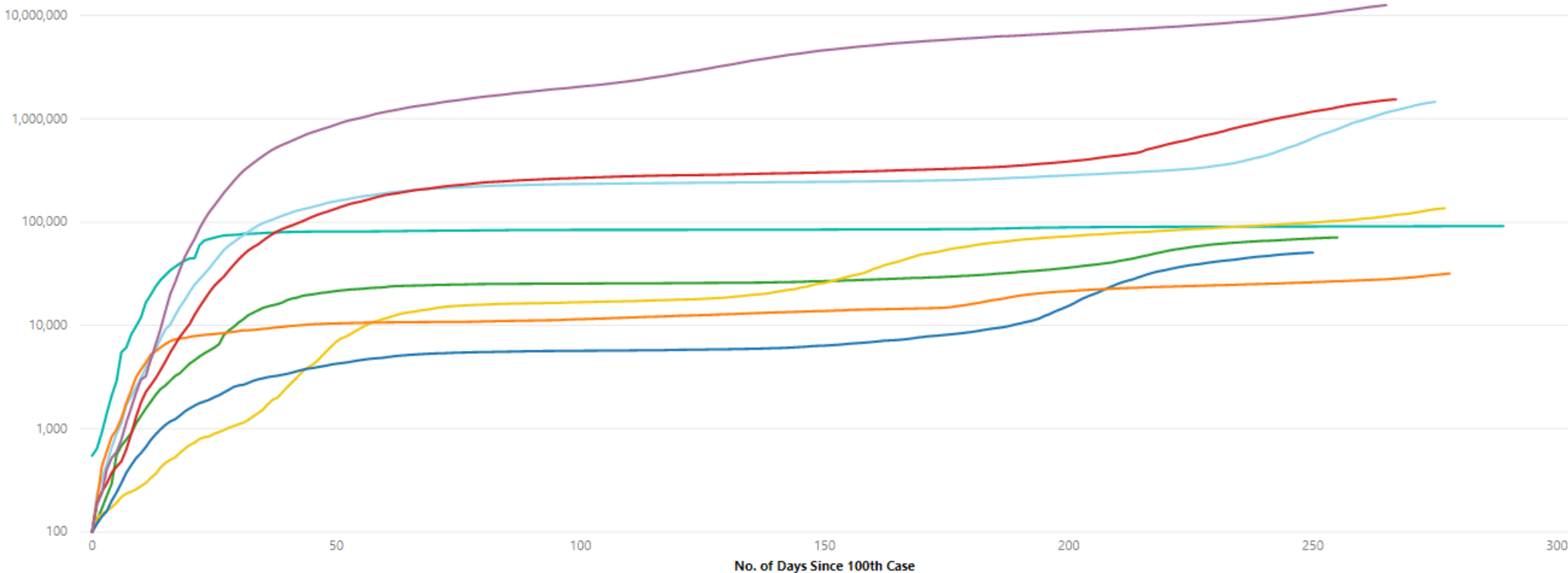
Cumulative Cases by Number of Days Since 100th Case
