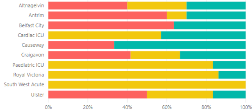
Covid-19 ICU Bed Occupancy : 5 Day Rolling Average
