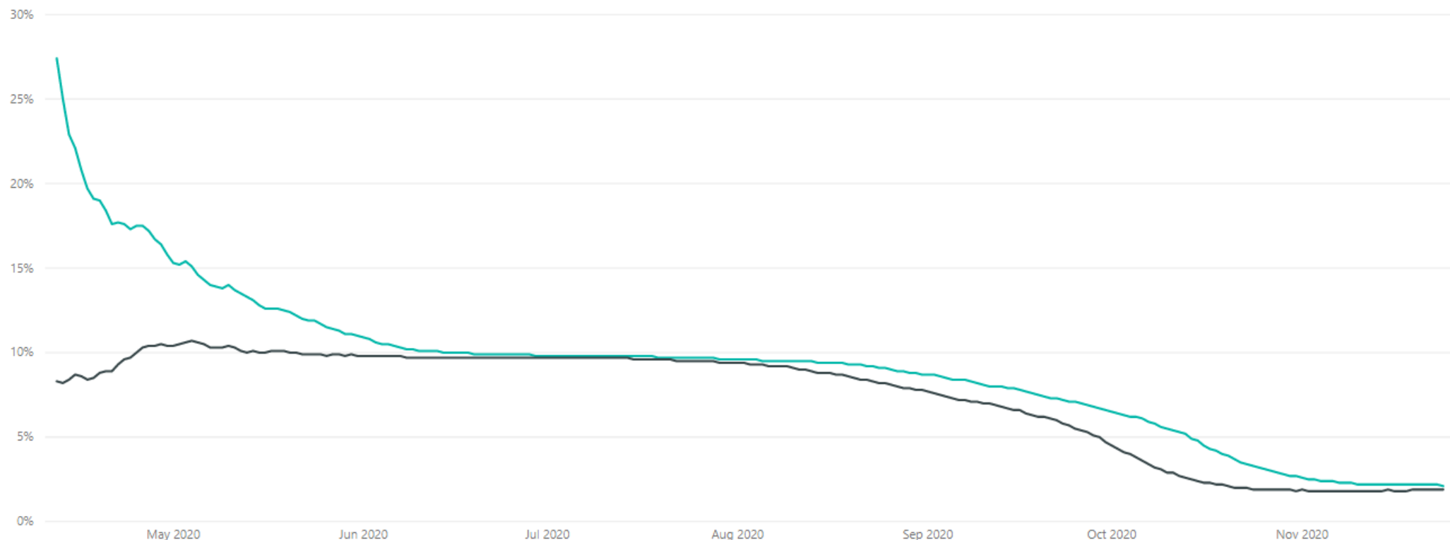
Figure 3: Mortality rate estimates are often based on the number of deaths relative to the number of confirmed cases, however, this isn't representative of the actual death rate, as patients who die on any particular day were infected much earlier. In other words, current deaths belong to the same group of patients that were infected in the past. The maximum incubation period for COVID-19 is assumed to be up to 14 days, therefore the chart below recalculates mortality by dividing the number of cumulative deaths at a specific date by the number of confirmed COVID-19 cases 14 days before.
