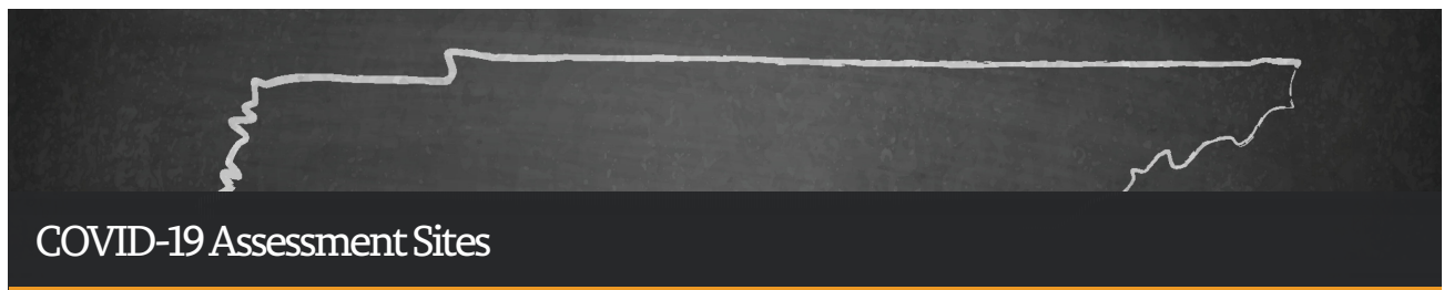
Novel Coronavirus
