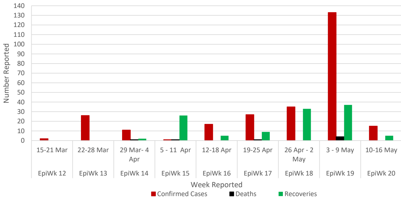
Figure 1: Weekly COVID-19 confirmed cases (N=267), deaths (N=7) and recoveries (N=117) as of 11 th May 2020
