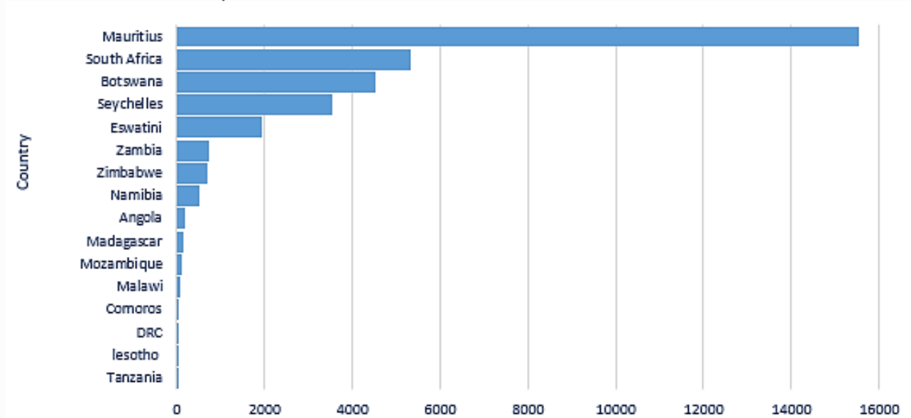
Figure 7: COVID-19 tests/million population by Country in Southern Africa (Source: Africa CDC dashboard), 10 th May 2020
