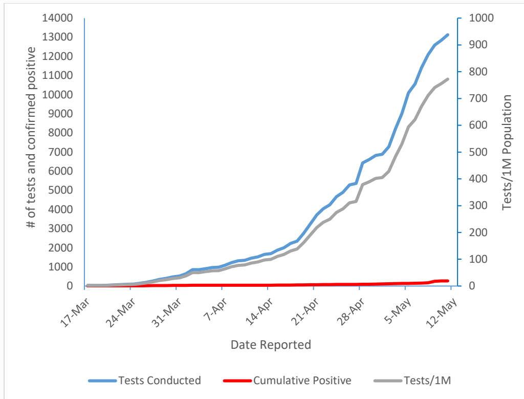
Figure 6: Graph showing cumulative number of PCR tests conducted, confirmed cases and tests per 1M population between 17 th March and 11 th May 2020
