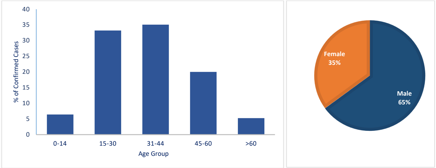
Figure 4: Age and Sex distribution of confirmed cases, as of 11 th May 2020
