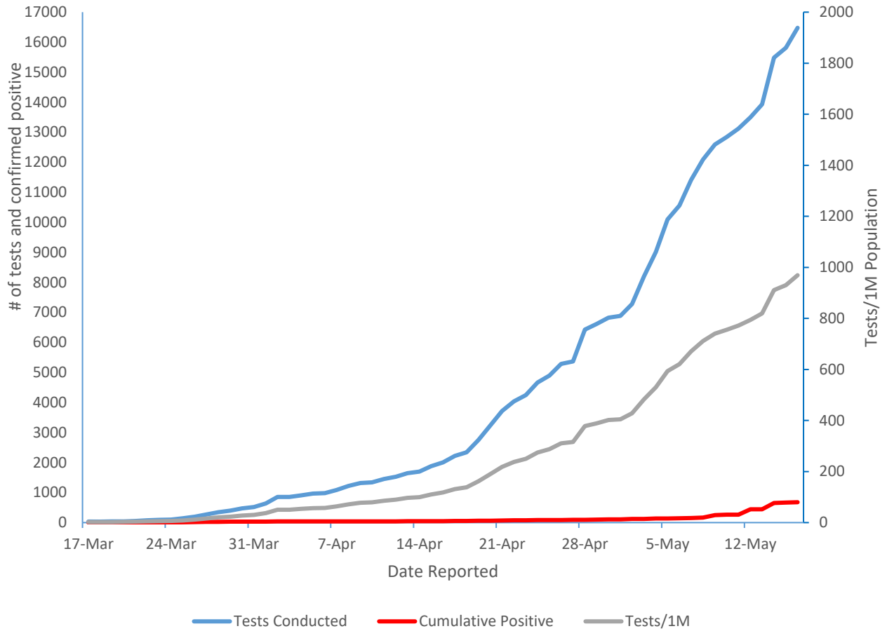
Figure 5: Graph showing cumulative number of PCR tests conducted, confirmed cases and tests per 1M population between 17 th March and 16 th May 2020
